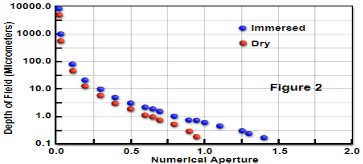
Depth of Field versus Numerical Aperture
