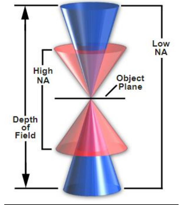
Depth of Field versus Numerical Aperture
